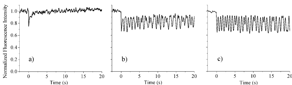
FIGURE 6 Fluorescence recovery signal for isolated nucleus stained with H333342 (a) at 400 mM NaCl, (b) for same nucleus as in a but after exposure to \sim 20 \text{ J/cm}^2 of 365 nm cross-linking light, (c) at 400 mM after exposure to 400 mM formaldehyde cross-linking conditions.
